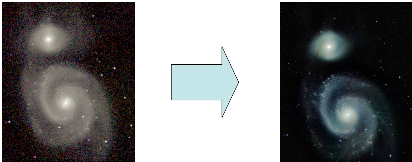
M51 from 2MASS (left, Jarrett et al., 2003) and from WFCAM, the camera used for UKIDSS (right, credit: Cambridge Astronomical Survey Unit)
